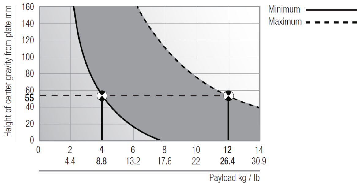
COUNTERBALANCE GRAPH
