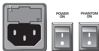
Fig. 5.5: Voltage supply and fuse
