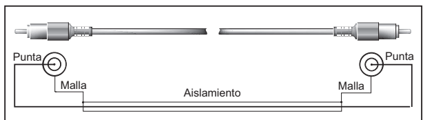
Fig. 5.3: Cable RCA
