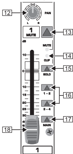
Fig. 2.4: Fader de canal, regulador Pan, interruptor Mute, etc.
