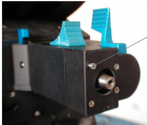
Position Pin on Tilt Gear Box
